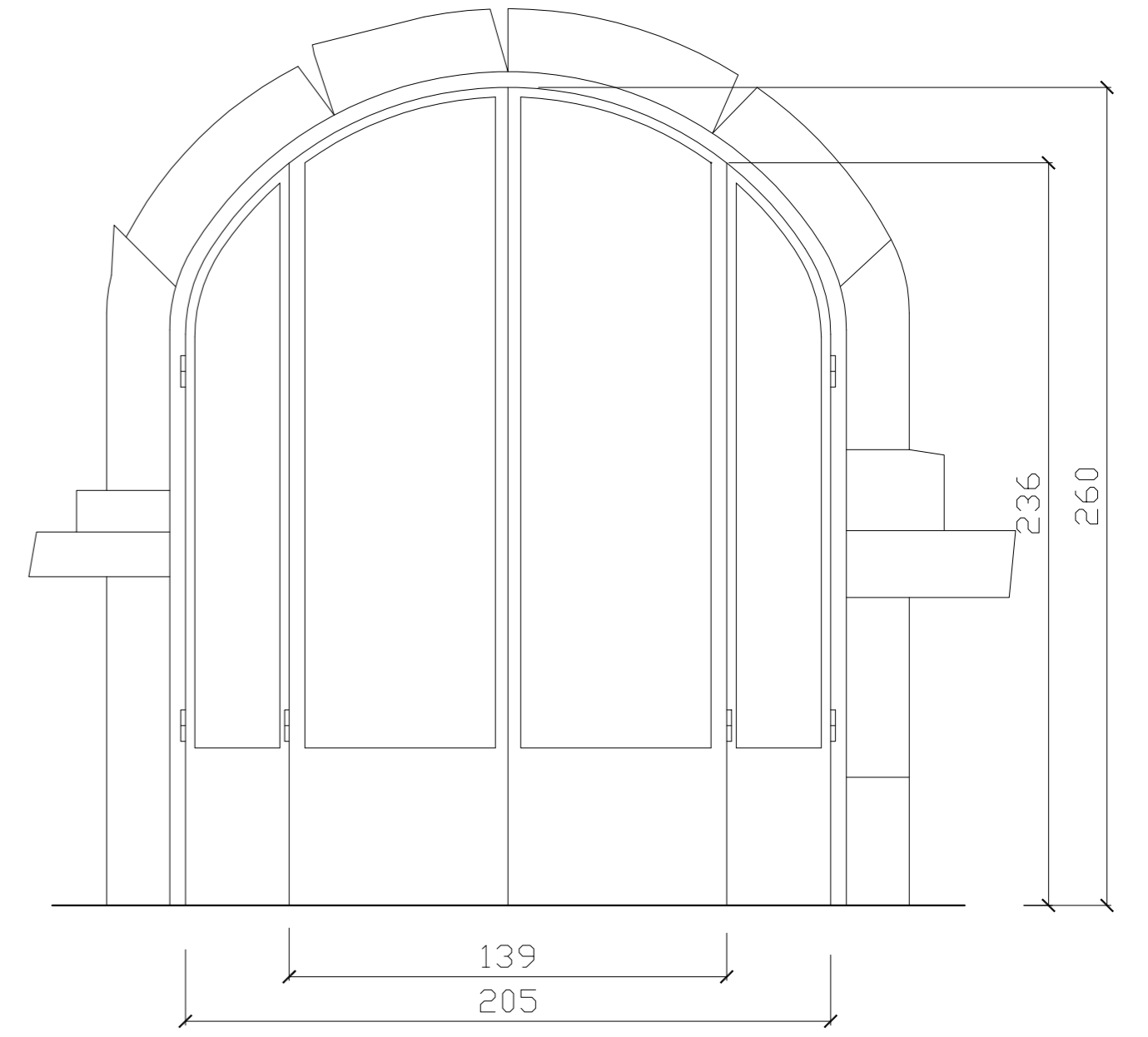
DETAIL B 1/20
